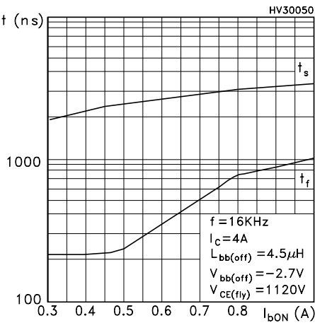
Figure 10. Inductive load switching time
